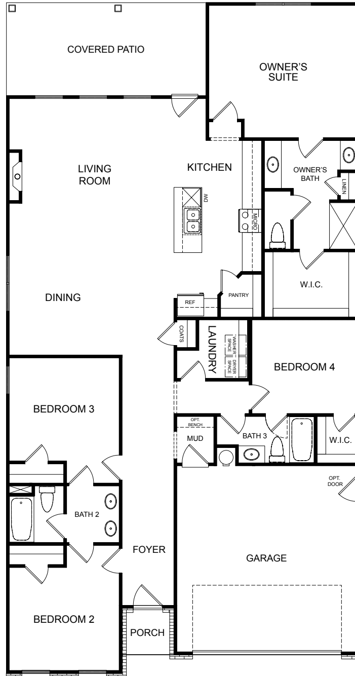
FIRST FLOOR
